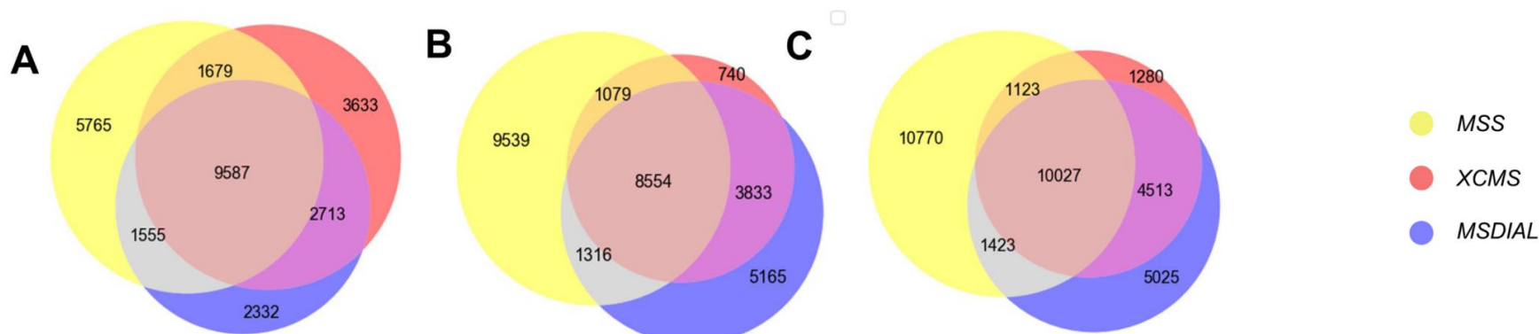
Fig. 2 Comparisons of feature extraction outcomes for identical input samples. Samples numbered A #505, B #506 and C #508 from the ENTACT study [73] with MSS, XCMS and MSDIAL software processing. Venn diagrams report extracted features overlap between different platforms. The feature extractions were performed with parameters matched as closely as possible across the different platforms. Key parameters for peak extraction for different platforms are reported in Additional file 1: Table S2
